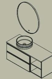
CONJUNTO 120 Assembly | Ensemble
